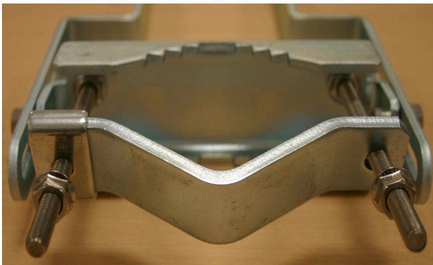
Figure 104 : Rear strap connected to upper AP antenna bracket
