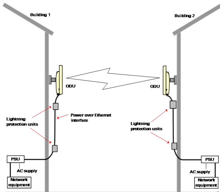
Figure 1: PMP/PTP 450 Platform Family typical bridge deployment
