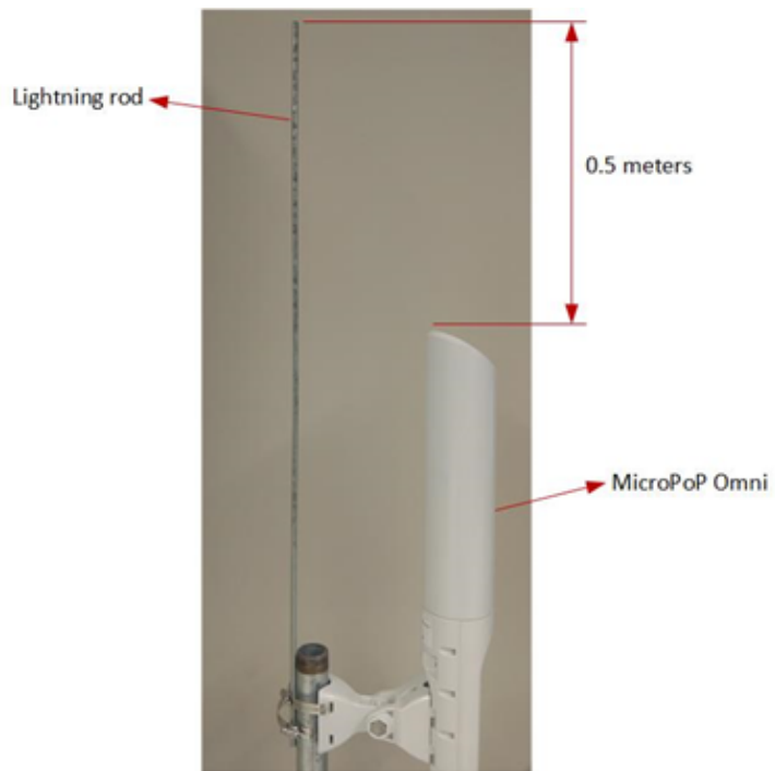
Figure 30 : MicroPoP Omni with Lightning rod
