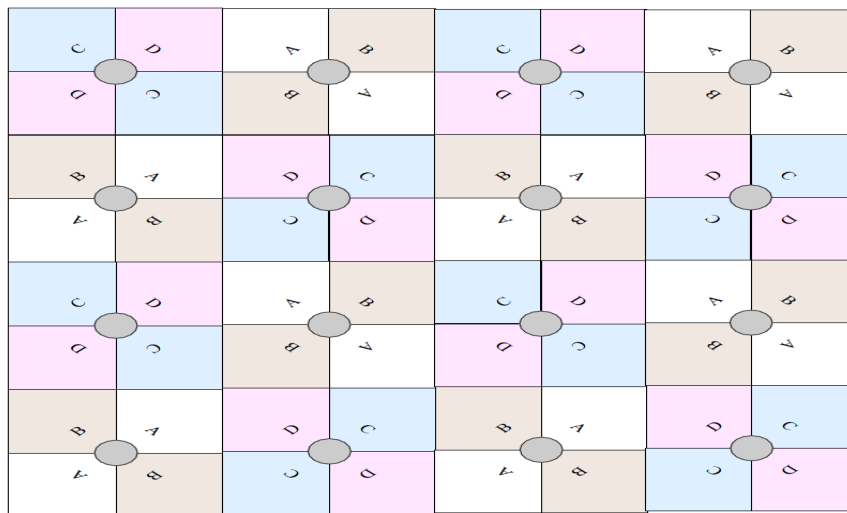
Figure 57 : Example layout of 16 Access Point sectors (ABCD), 90-degree sectors
