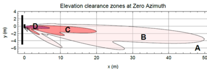
Figure 60 : Sector Antenna
