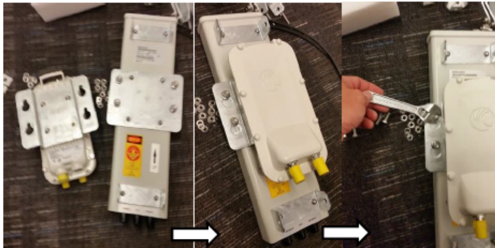
Figure 92: Attaching the plate
