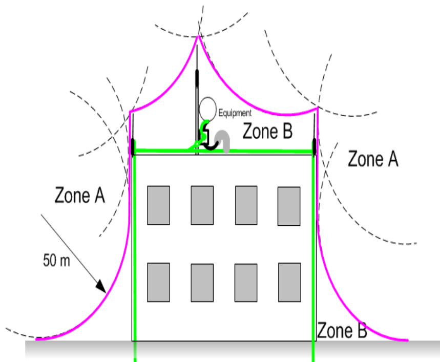
Figure 56 : Rolling sphere method to determine the lightning protection zones
