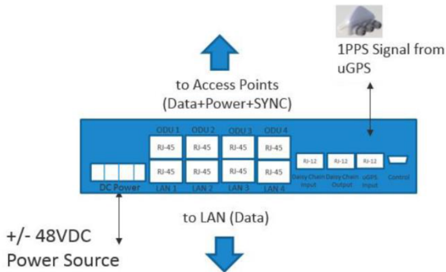
Figure 40 : Cluster Management: Scenario 1
