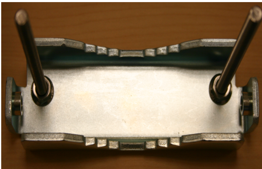
Figure 102 : AP antenna upper bracket assembly
