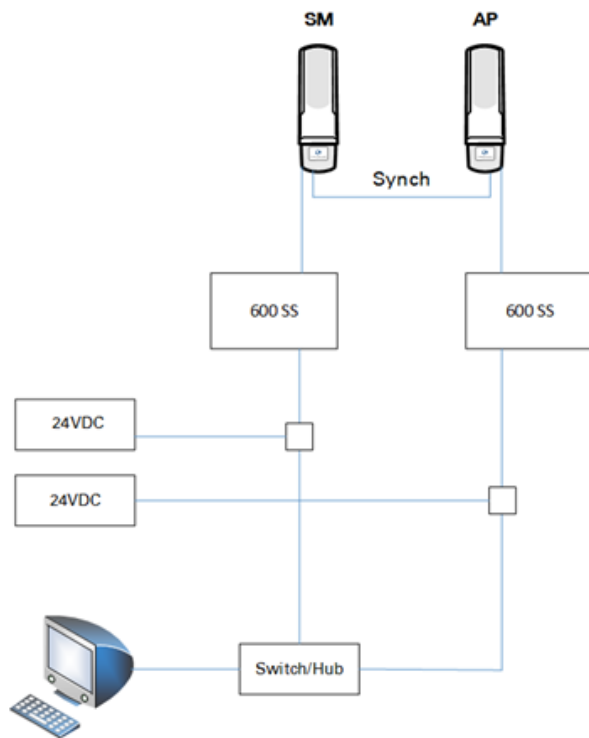
Figure 68 : Remote AP wired to SM that also serves a customer
