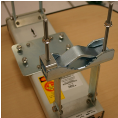
Figure 107 : Lower bracket attached to AP antenna
