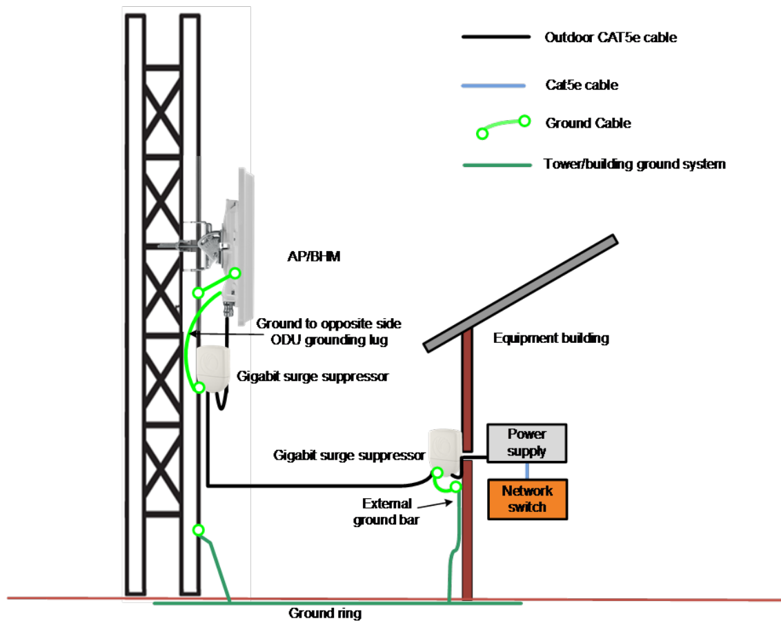
Figure 85 : Grounding and lightning protection on mast or tower
