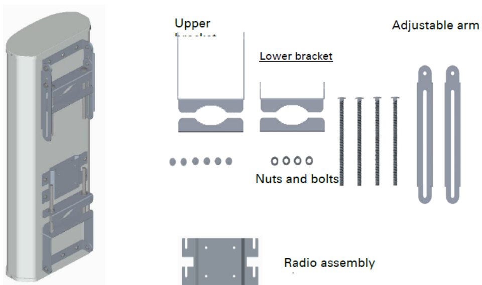
Figure 115 : PMP 450i AP 900 MHz antenna inventory
