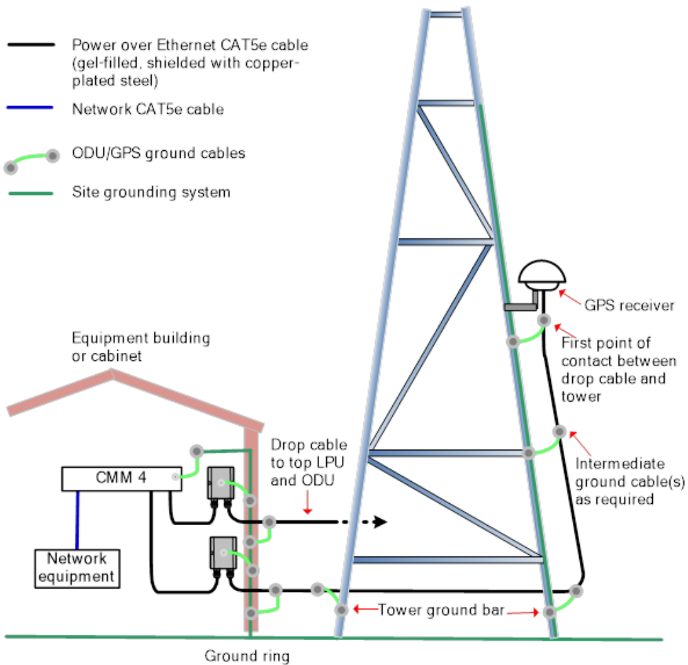
Figure 55 : GPS receiver tower or mast installation
