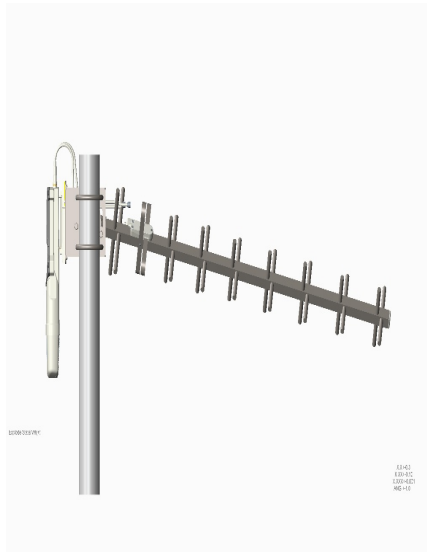
Figure 125 : Yagi antenna alignment - downward tilt
