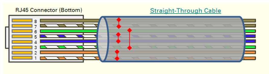
Figure 88 : RJ45 cable
