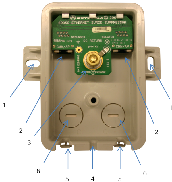
Figure 82 : 600SSH Surge Suppressor – inside
