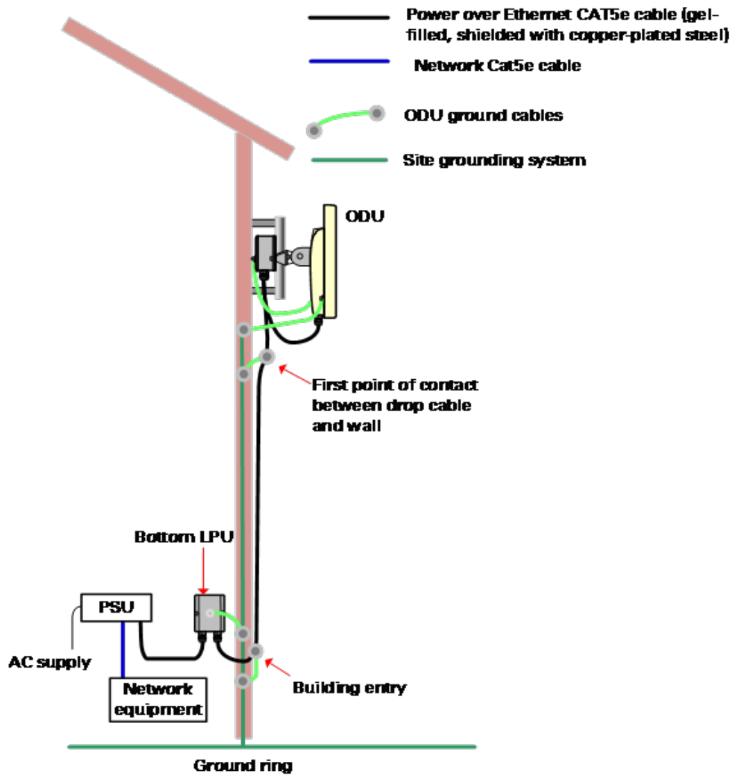
Figure 52 : Wall installation
