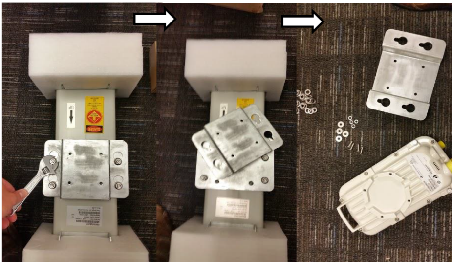
Figure 90 : Antenna top plate
