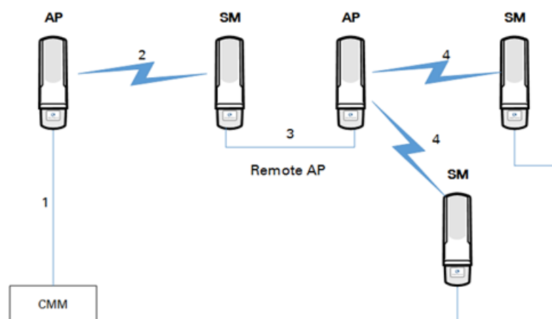
Figure 70 : Additional link to extend network sync, Design 3
