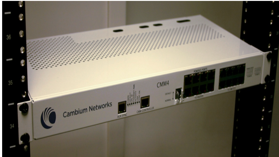
Figure 44 : CMM4 (Rack Mount)
