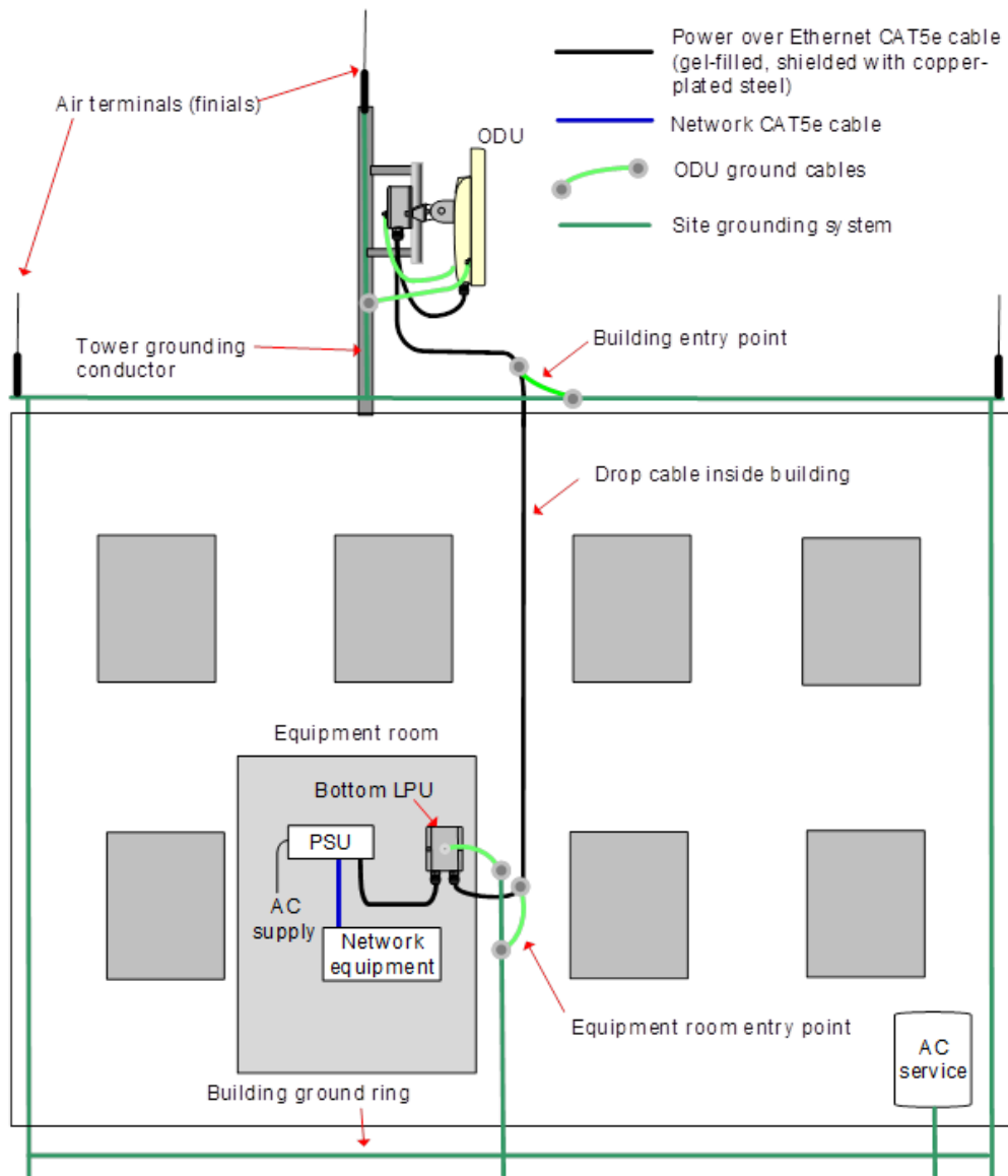
Figure 53 : Roof installation
