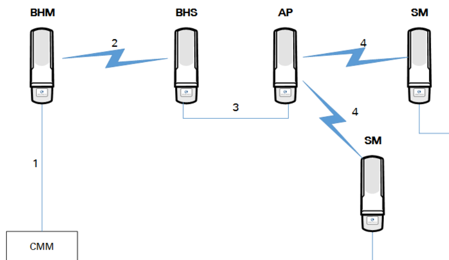
Figure 72 : Additional link to extend network sync, Design 5
