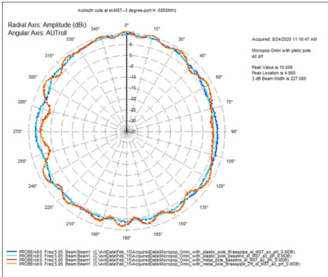
Figure 28 : MicroPoP Omni antenna implementation pattern (Horizontal)
