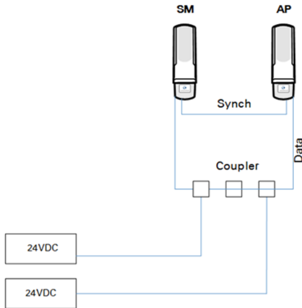
Figure 69 : Remote AP wired to SM that serves as a relay
