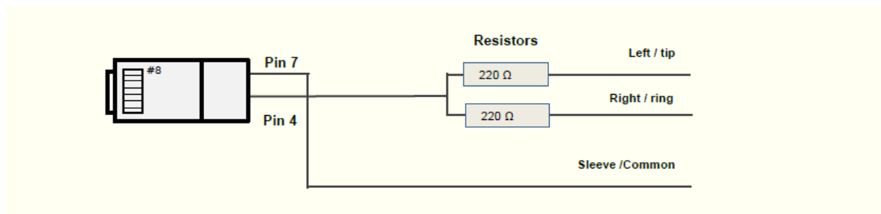
Figure 34 : Alignment Tone Cable
