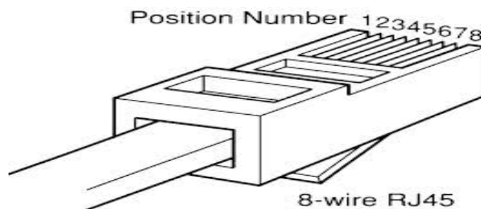
Figure 74 : Pin 1 location
