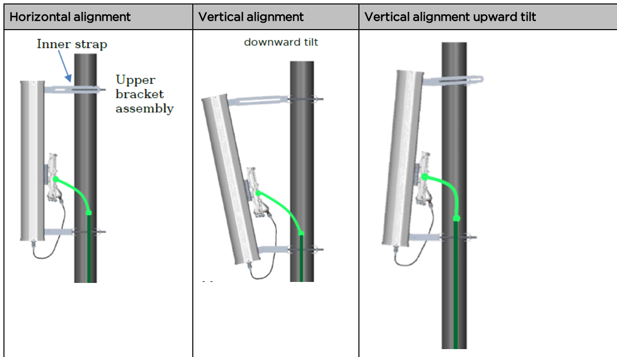
Figure 117 : 900 MHz sector antenna alignment
