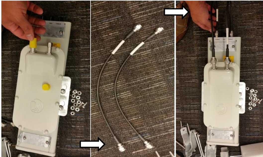
Figure 93 : Connect the port A and B to the PMP 450i AP
