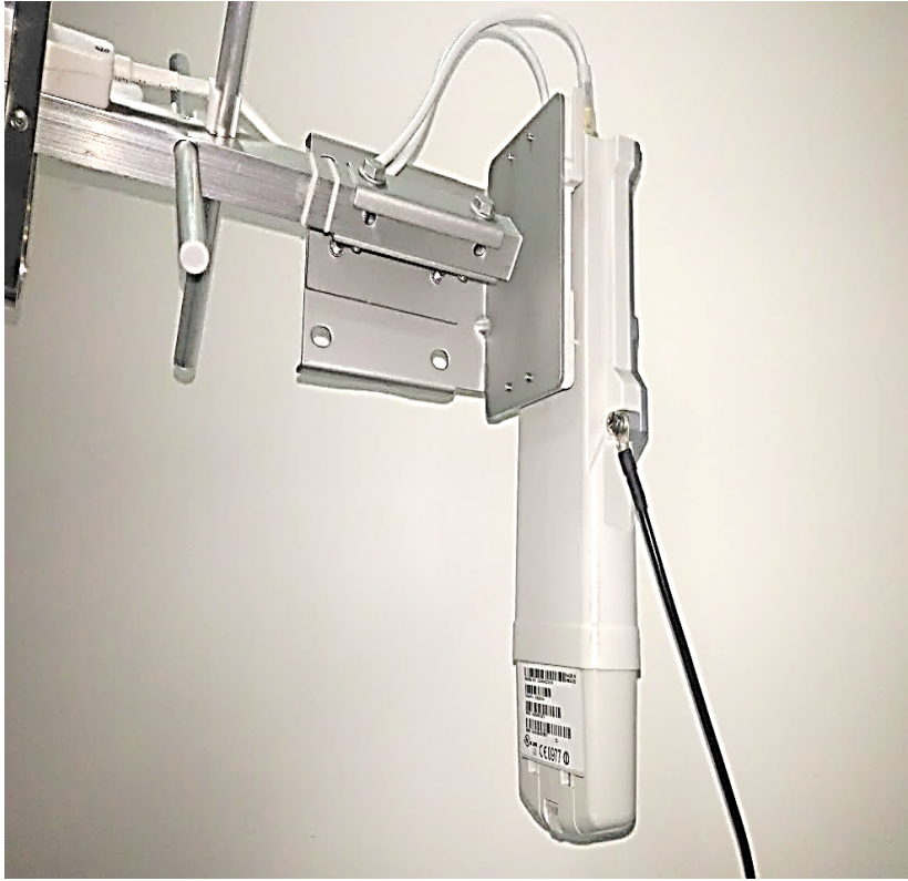
Figure 80 : PMP 450 900 MHz SM grounding
