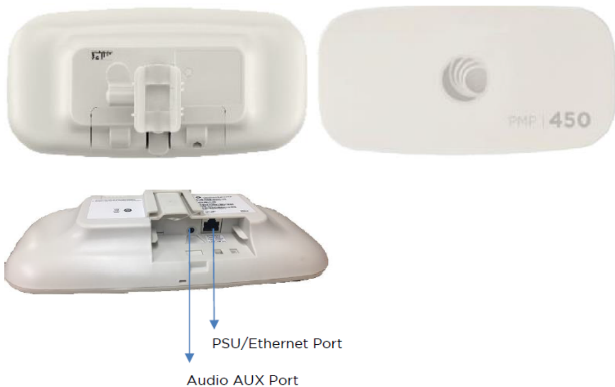
Figure 6 : PMP 450b Mid-Gain Series - SM interfaces
