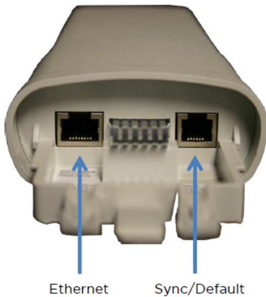
Figure 10 : PMP/PTP 450 Series – SM/BH Connectorized interfaces
