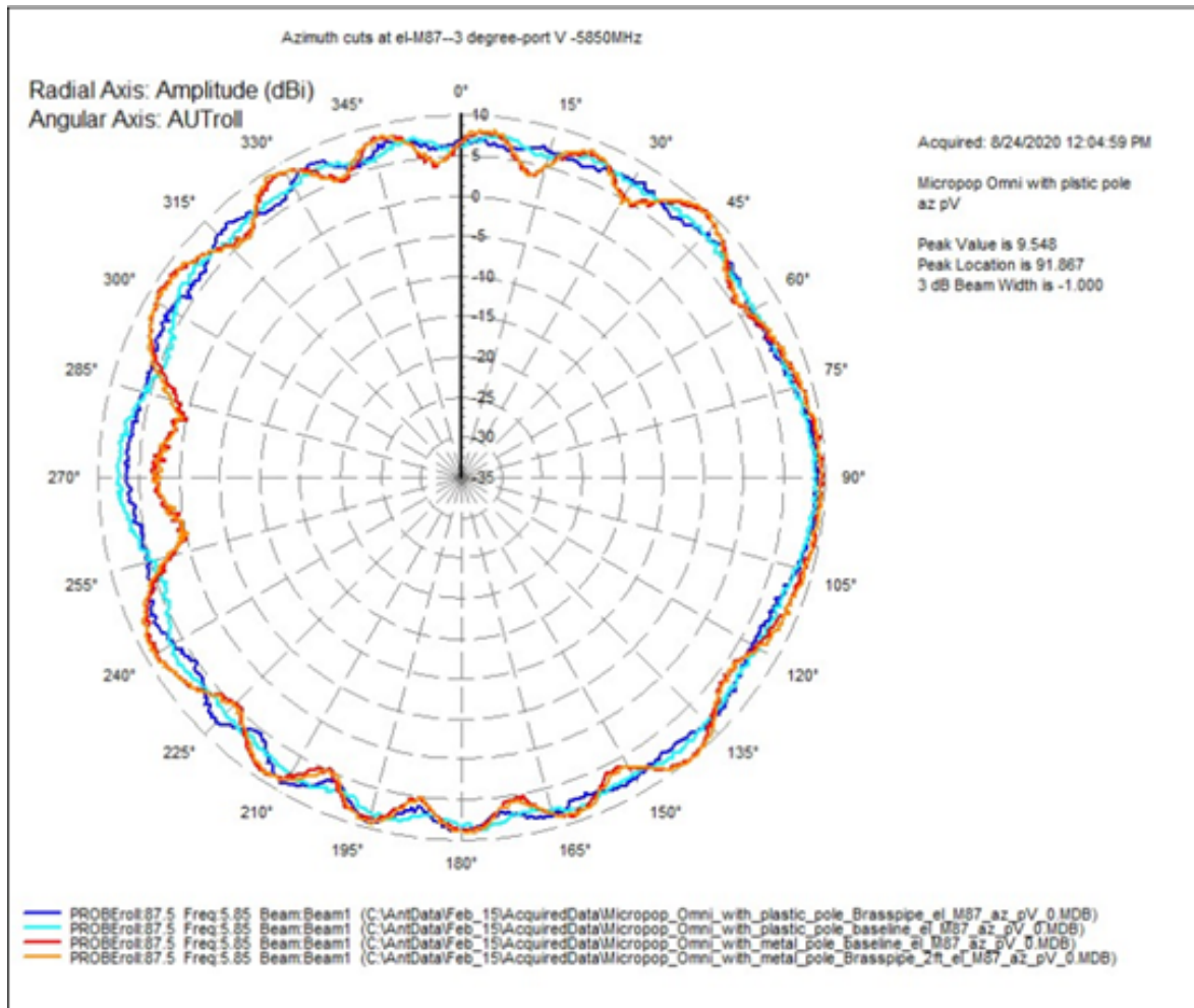
Figure 29 : MicroPoP Omni antenna implementation pattern (Vertical)
