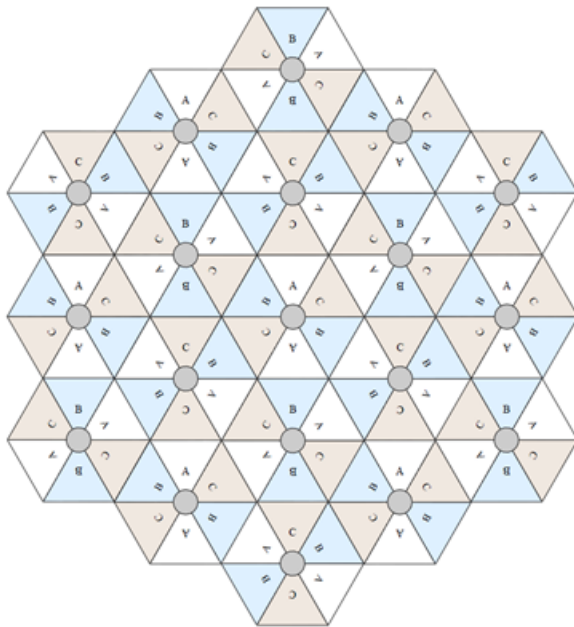
Figure 58 : Example layout of 6 Access Point sectors (ABC), 60-degree sectors
