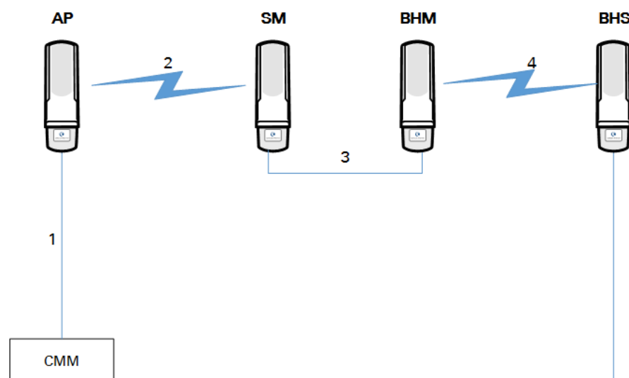
Figure 71 : Additional link to extend network sync, Design 4
