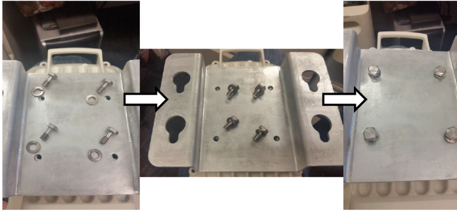
Figure 91: Attaching antenna plate to the AP
