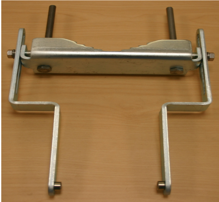
Figure 95 : AP antenna upper bracket attached to upper adjustment arms
