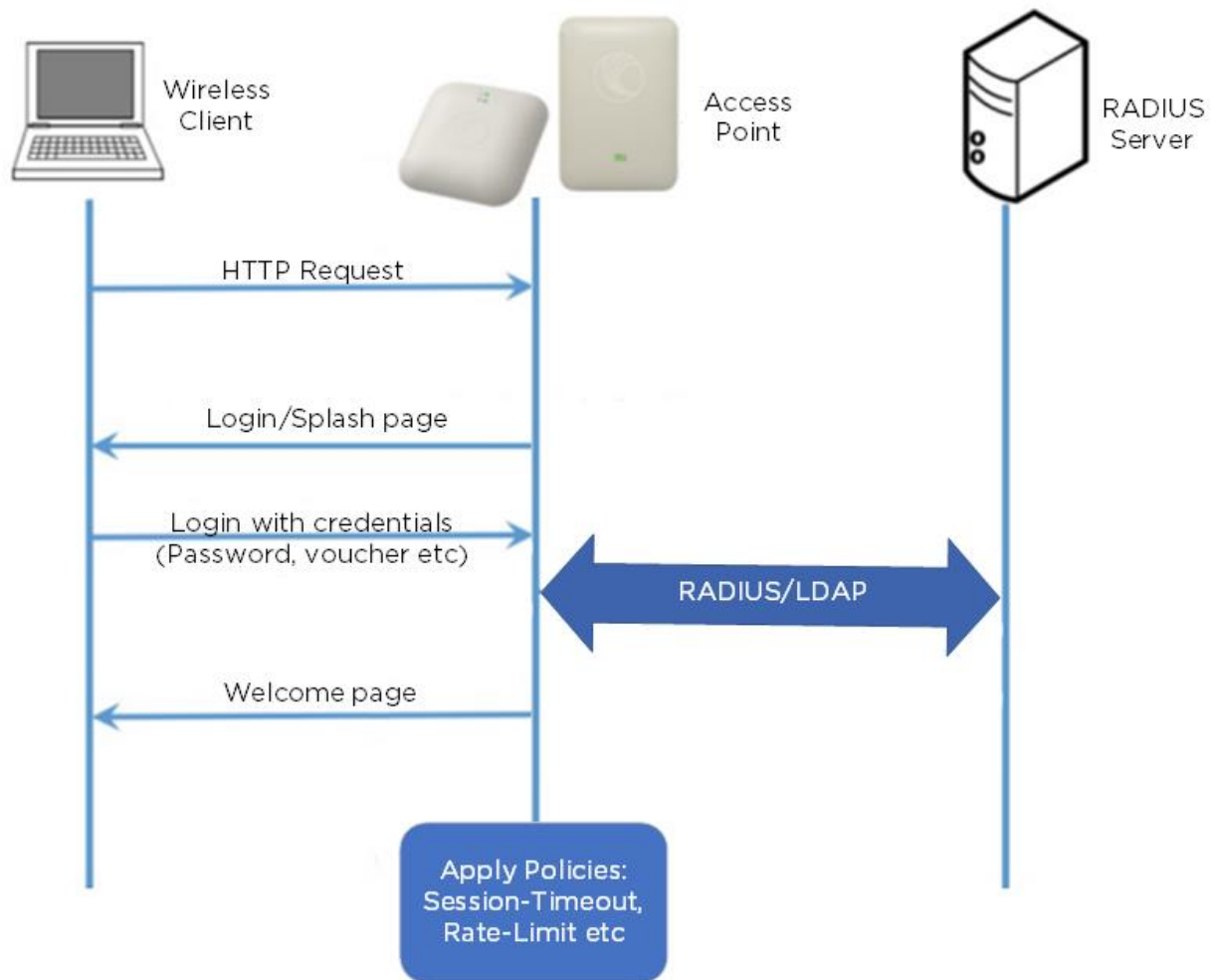
Figure 89 Topology
