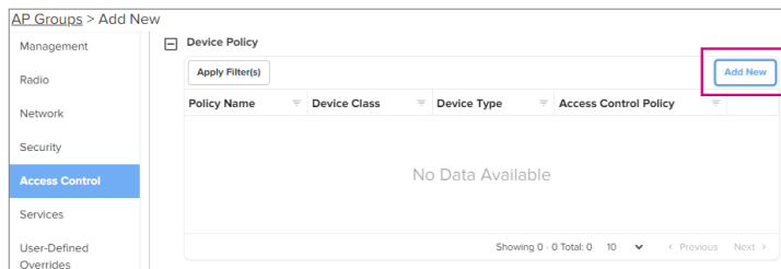
Figure 51 Device Policy
