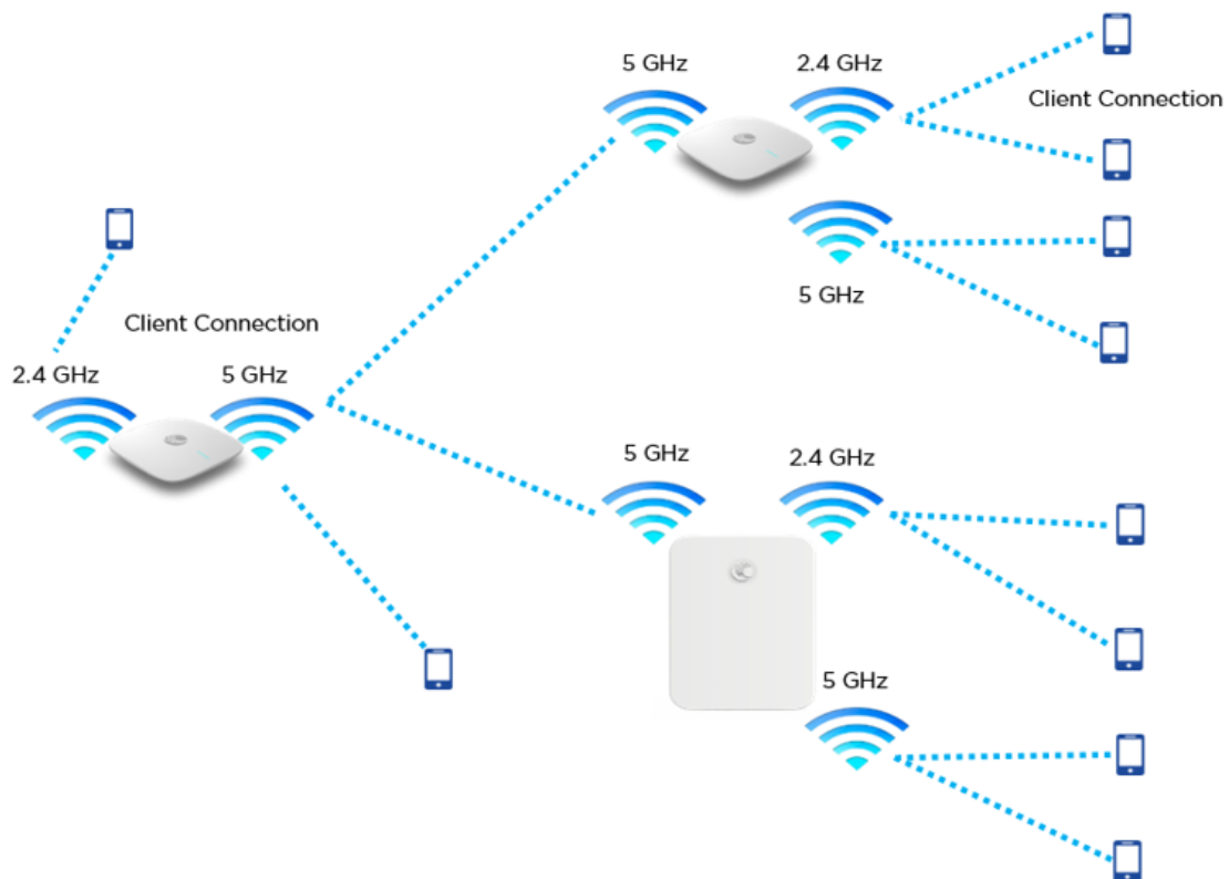
Figure 83 Single hop mesh connection in 5 GHz with two Mesh Clients and 2.4 GHz and 5 GHz as access
