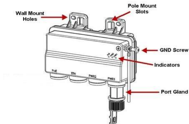
Figure 8: PoE Injector
