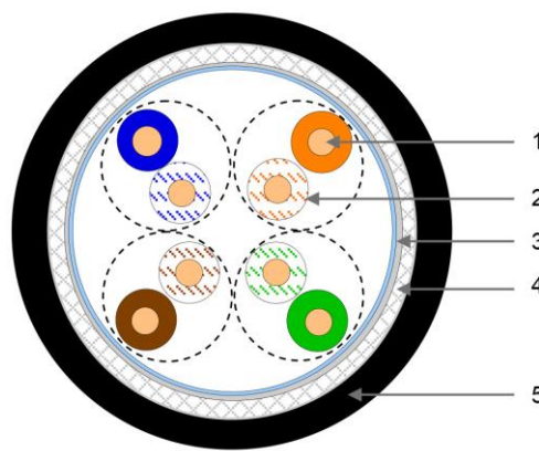
Figure 17: Cable Design
