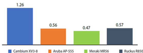
Wi-Fi 6 8x8 MIMO Access Points Price-Performance Ratio (Mbps/Dollar)
