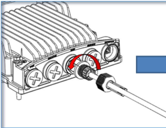
Tightening the Front Portion of the Gland
