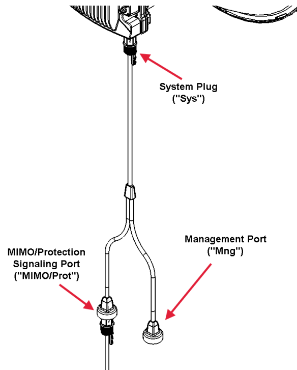
Figure 15 MIMO/Protection signaling cable 2
